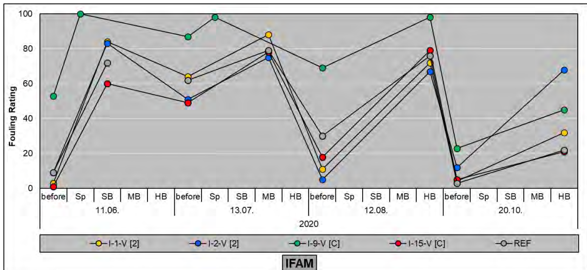
Fig.31: ASTM fouling rating at wear testing (IFAM) at Norderney beachside sublittoral at four inspections in 2020 before and after 30 s cleaning by sponge, soft, medium, or hard brush.
