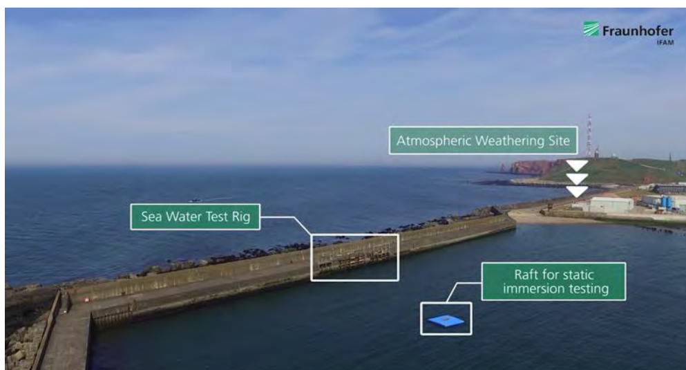
Fig.14: Overview of the Fraunhofer IFAM test stands on Helgoland
