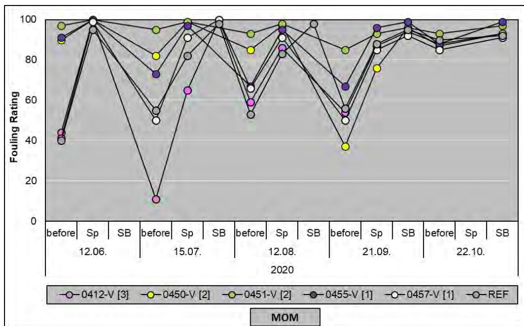
Fig.21: ASTM fouling rating at wear testing of coatings (MOM) in Norderney harbour at five inspections in 2020 before and after 30 s cleaning by sponge or soft brush.
